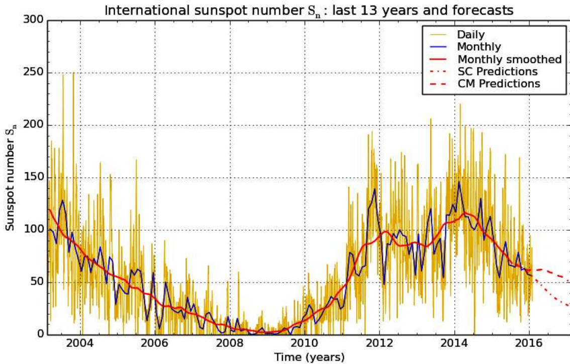
SILSO graphics ( http://sidc.be/silso ) Royal Observatory of Belgium 2016 February 1
