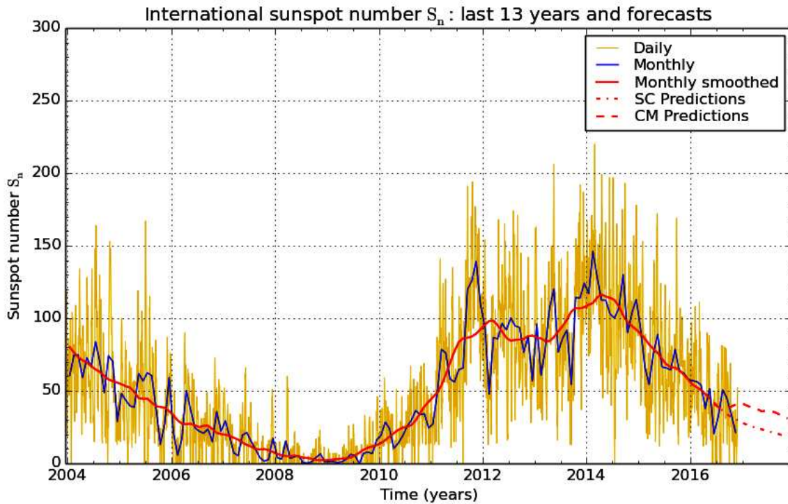
SILSO graphics ( http://sidc.be/silso ) Royal Observatory of Belgium 2016 December 1
